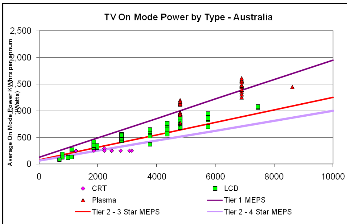
Figure 8 Television Power Consumption – Australian Data Set
