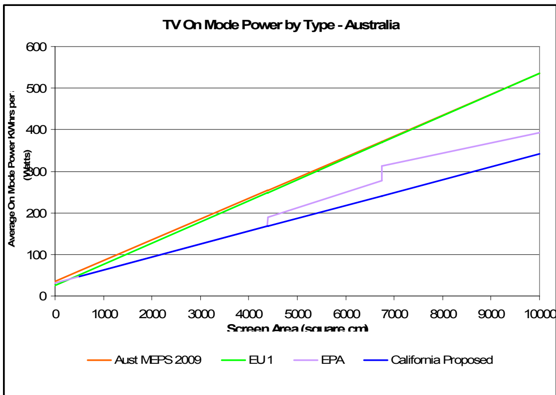
Figure 19: Comparison between Aust and other international Programs
