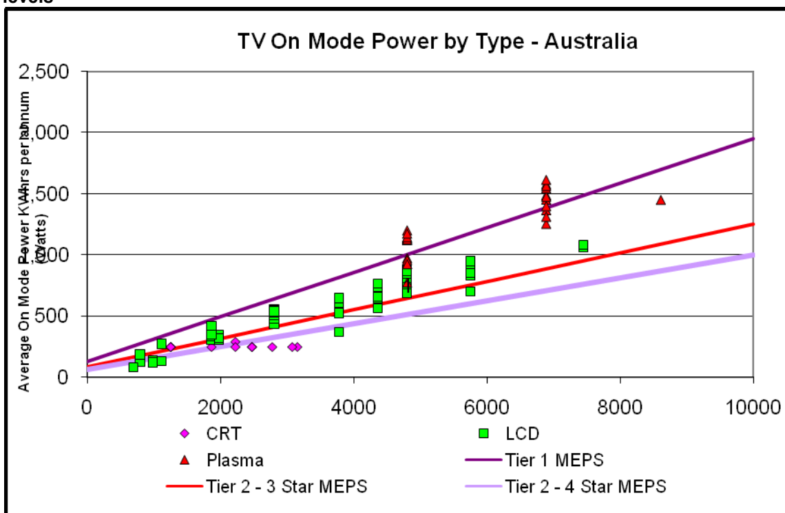
Figure 14 Comparison of Products 2007/08 in Australia against the Proposed MEPS levels
