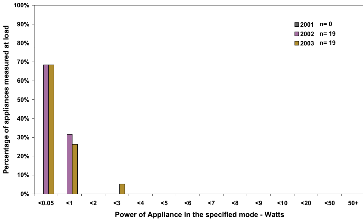
Figure 29 – Power measurements for AV receivers: off mode
